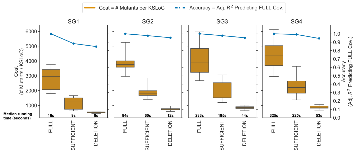
Figure 3: Cost and accuracy of the FULL, SUFFICIENT, and DELETION subsets of mutation operators, for each of the submission groups. For each subplot, the left axis represents cost (# mutants per KSLoC) and the right axis represents accuracy (adjusted R^2 in a model predicting FULL coverage). The y-axes are shared across subplots. Inline text at the bottom of the charts indicates the median running time on our server.
